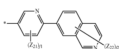
Formula 7-5
