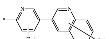
Formula 7-9
