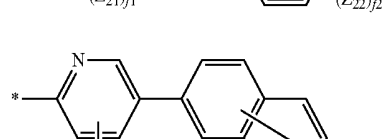
Formula 7-12
