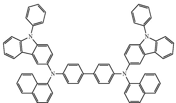
HT18
