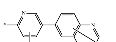
Formula 7-10
