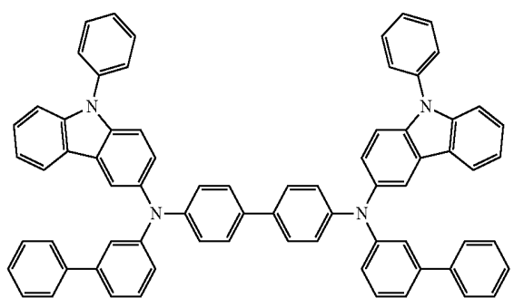
HT19
