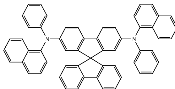
Spiro-NPD
