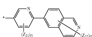
Formula 7-4
