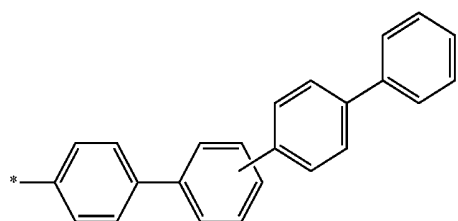
Formula 6-16
