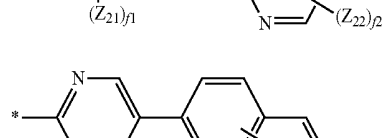
Formula 7-14
