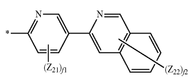
Formula 7-8
