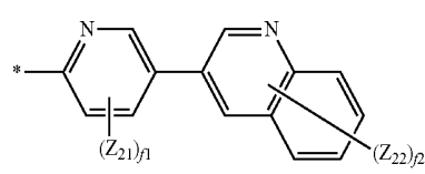
Formula 7-9
