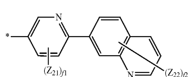
Formula 7-6
