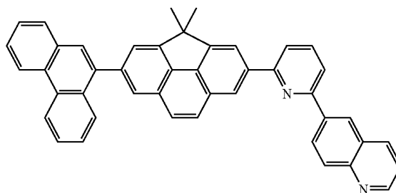
Compound A
