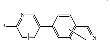
Formula 7-11
