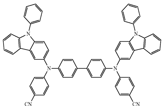
HT17
