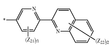
Formula 7-7
