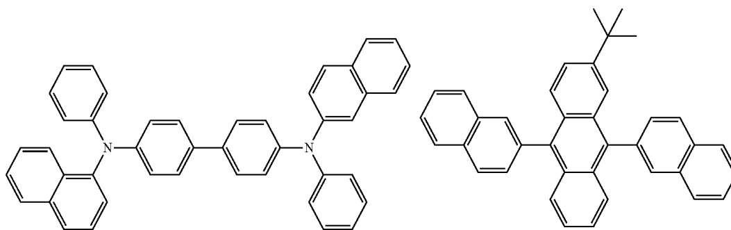
NPB
