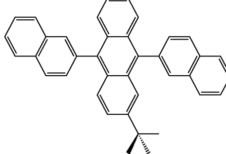
TBADN
