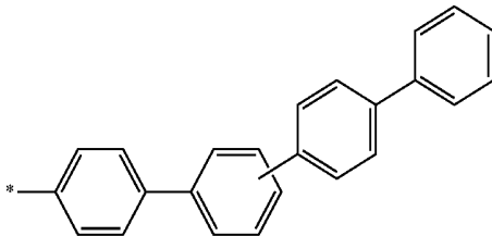
Formula 6-16
