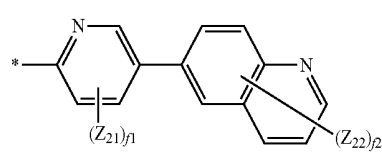
Formula 7-10
